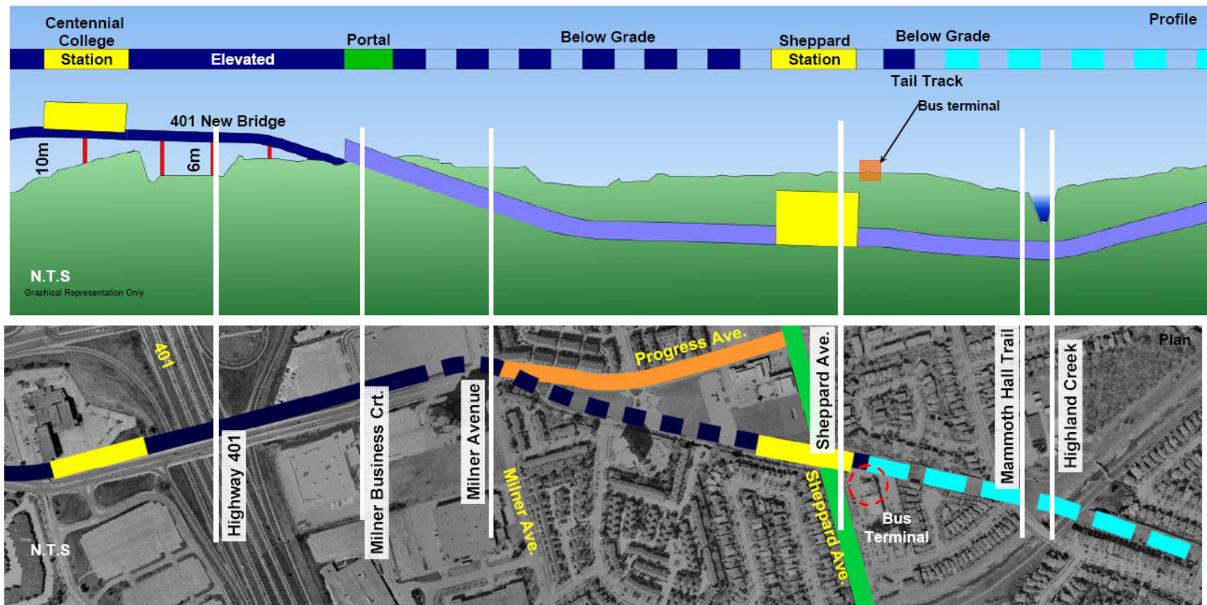
Exhibit E3-1: SRT Extension Alignment (Continued)
