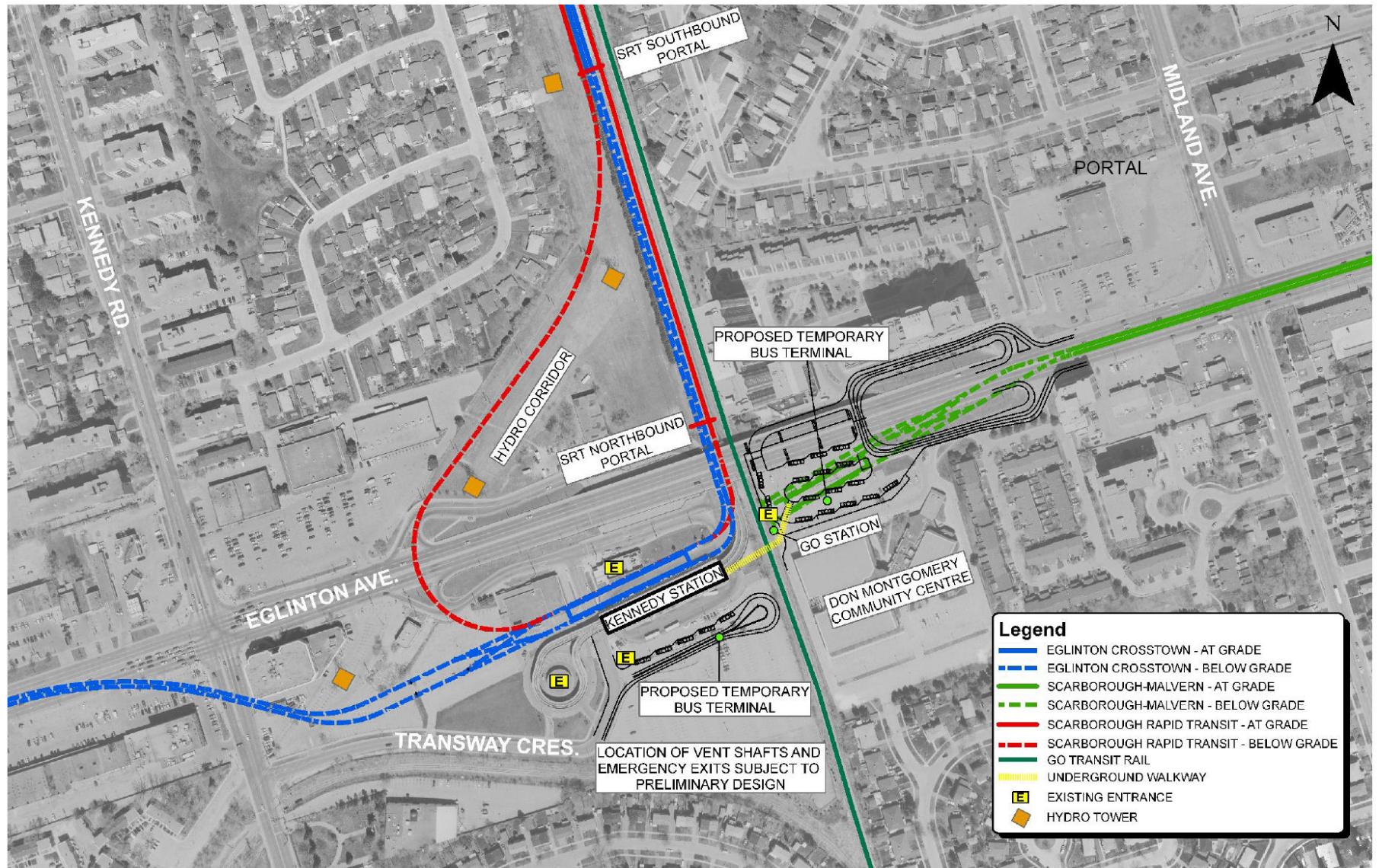
Exhibit 4- Kennedy Station Improvements – Plan
