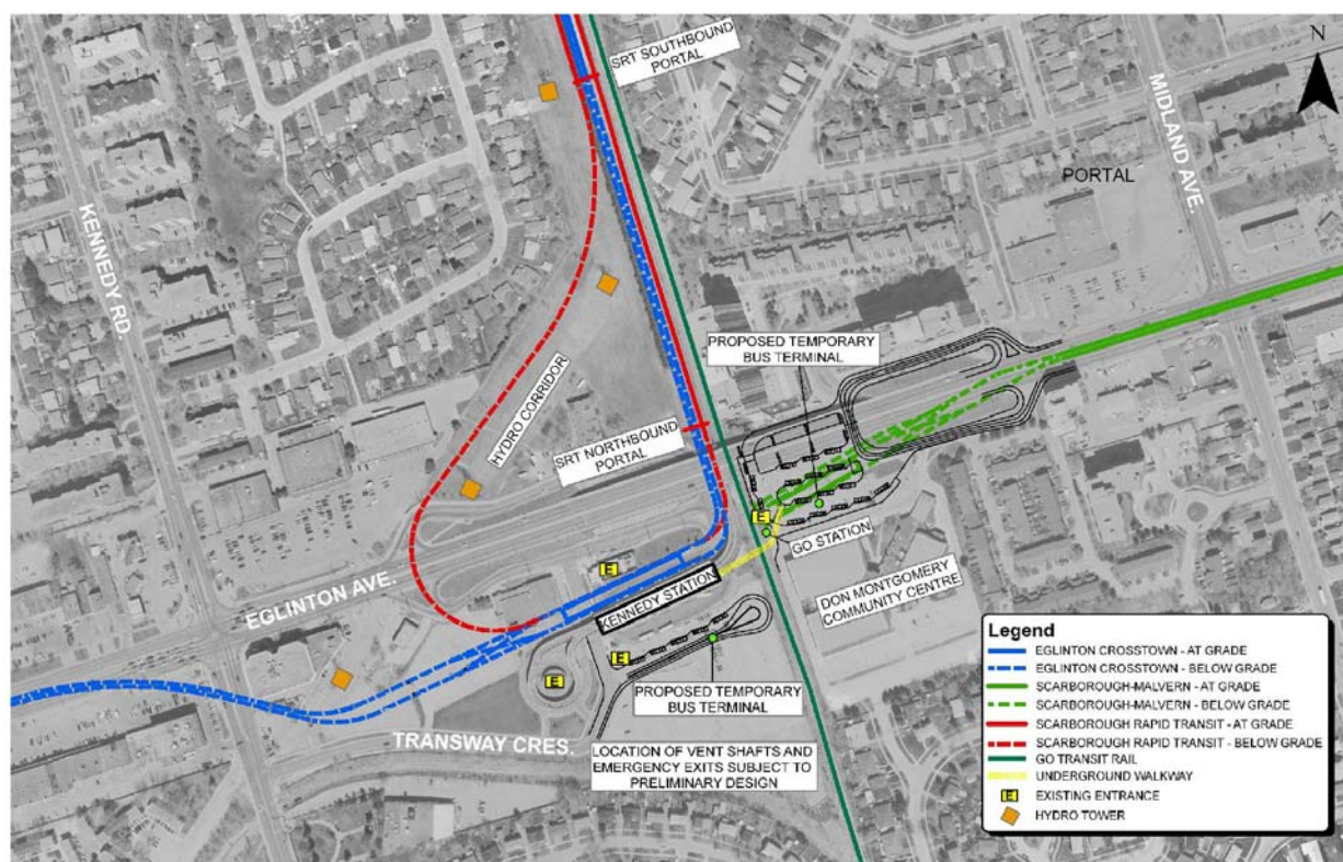
Exhibit E2-1: Kennedy Station
