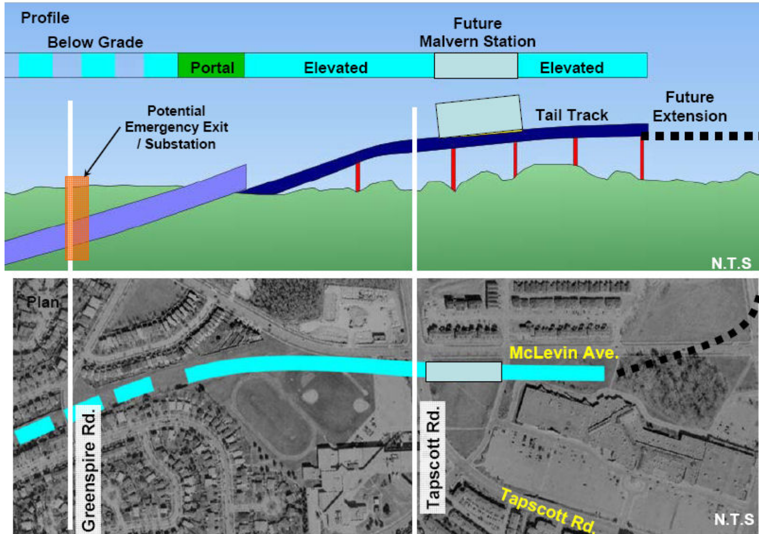
Exhibit E3-1: SRT Extension Alignment (Continued)
