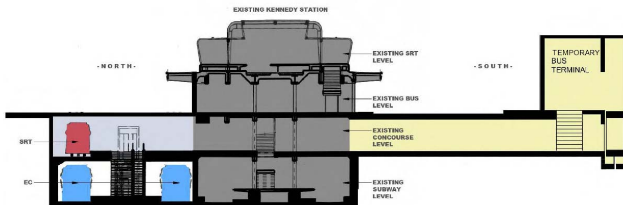
Exhibit E3-2: Kennedy Station – Cross-Section
