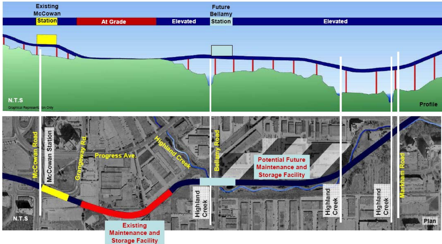
Exhibit E3-1: SRT Extension Alignment
