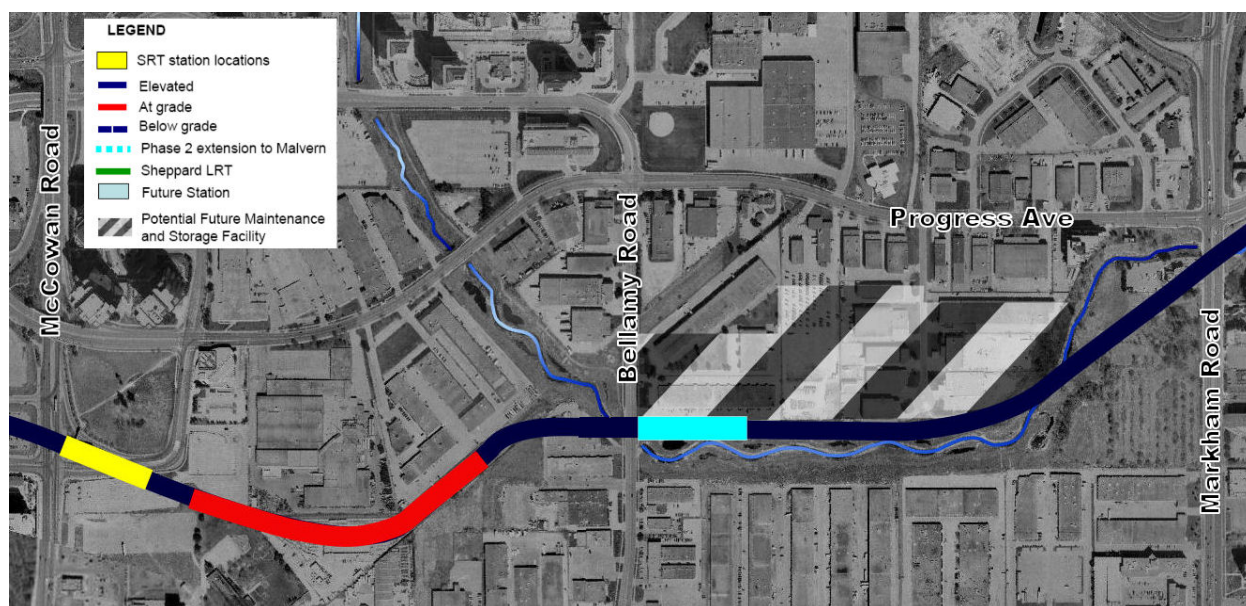
Exhibit E2-2: Preferred Alignment – McCowan Road to Markham Road
